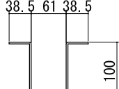
母屋取付板B t=2.3
