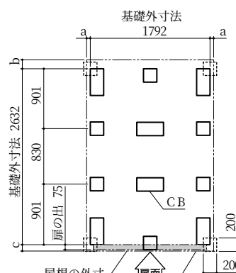
MBW-50CA・50CHA
